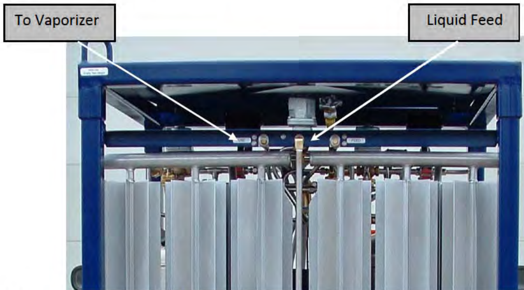
Figure 7 - Attachment Piping
