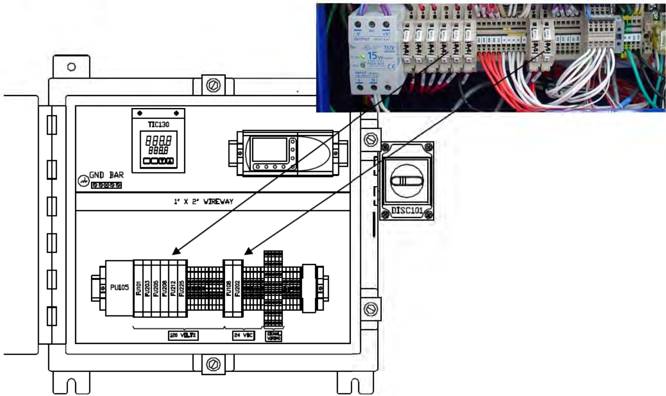
Figure 8 - Fuse Detail
