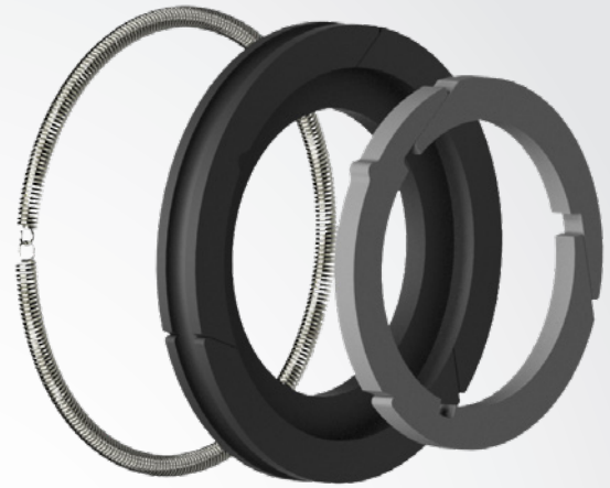
Exploded view of a double acting EMISSIONGUARD TR 2 packing ring
