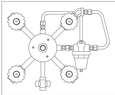
New MCR Regulator Plumbing Configuration
