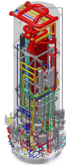
10 Tons/Day Hydrogen Liquefier Vacuum Cold Box – Inventor Model
