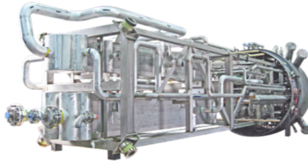
Helium Liquefier Vacuum Cold Box – 1800 Liters/Hr – Internal Assembly
