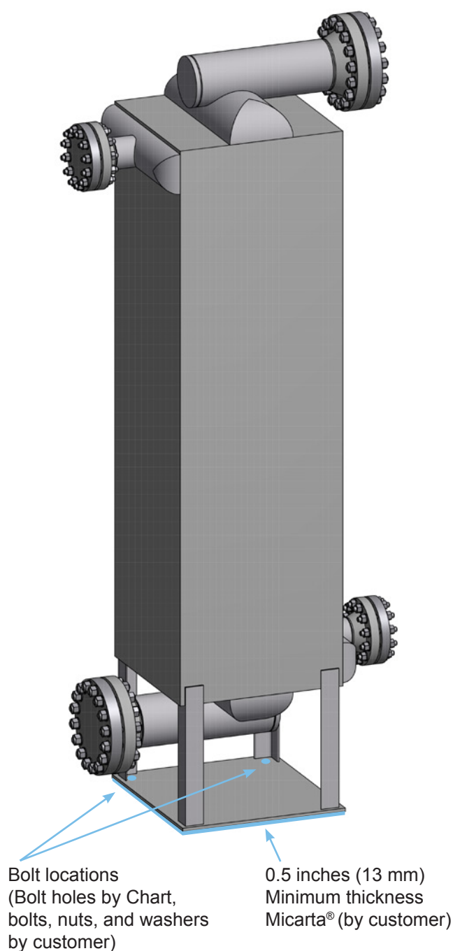
Typical pedestal base mounting system (Single or multiple BAHX assemblies) Warm end up (typical)
