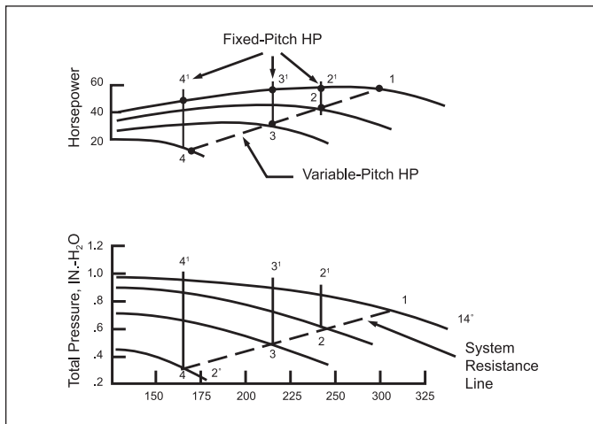
Throttled Flow Through Fan Fig. 19
