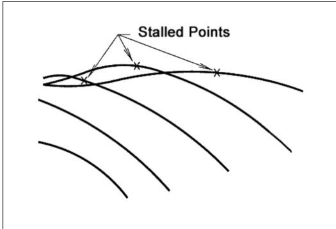
Stall Points on Fan Curve Fig. 4
