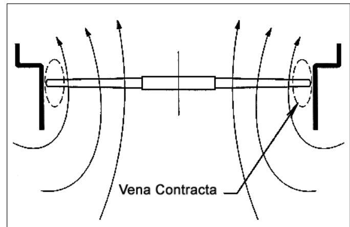
Airflow with No Inlet Bell Fig. 7
