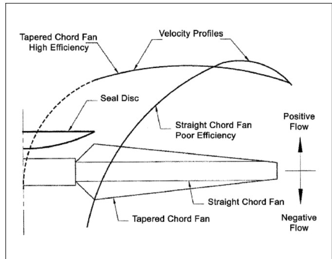
Velocity Profiles - Tapered vs. Constant Chord Blade Fig. 12
