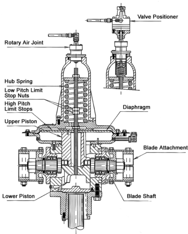
Typical Auto-Variable® Hub Fig. 18
