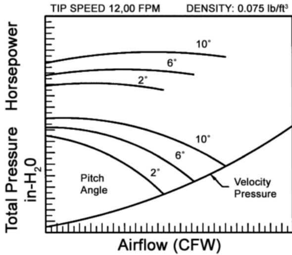
Typical Fan Curve Fig. 2
