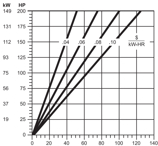
Approximate Cost of Power to Operate 8400 hrs/yr Fig. 10
