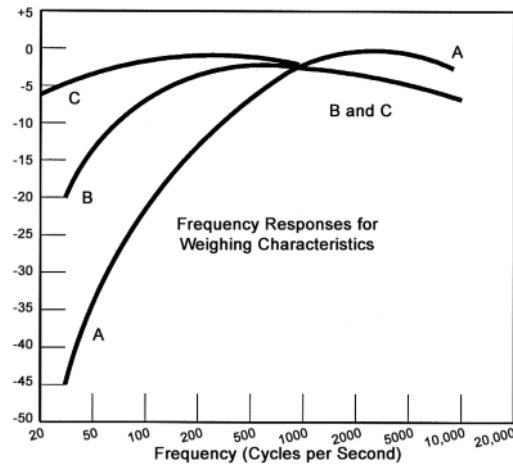
Weighted Sound Levels Fig. 22
