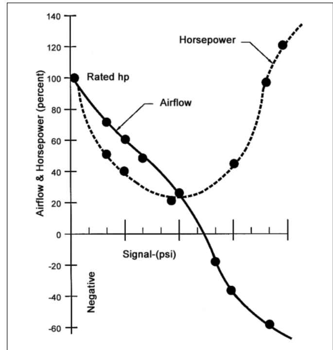
Airflow vs. Signal for Variable-Pitch Hub Fig. 17
