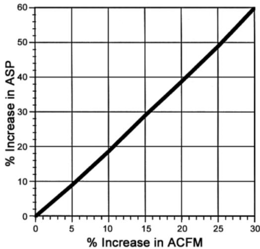
ASP vs. CFM for ACHE Fig. 11
