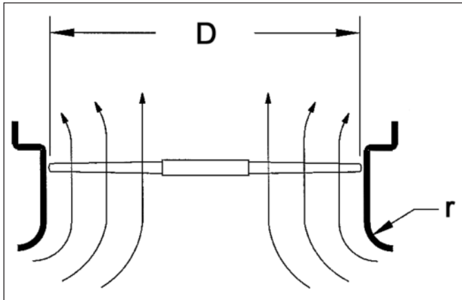
Airflow with Inlet Bell Fig. 8
