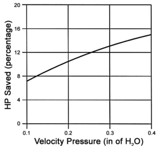
Approximate HP Savings with VR Fig. 3
