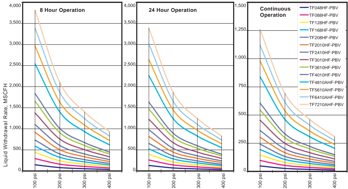
Liquid N 2 Withdrawal Ratings for Vertical Pressure Build Vaporizer Models
