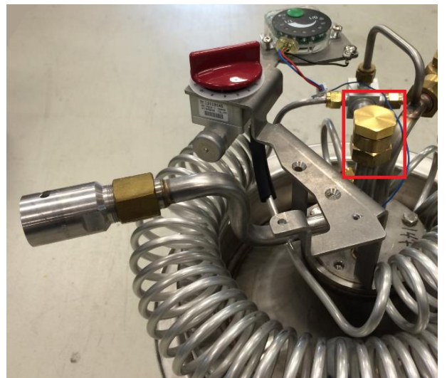
Figure 8. Newer Style Side Fill without Shroud
