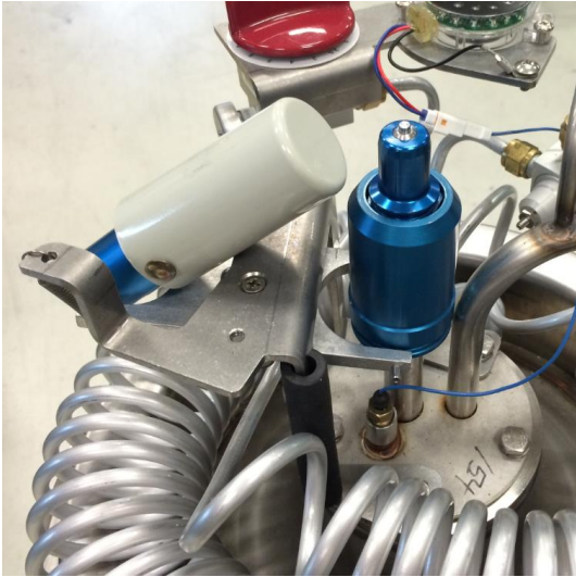
Figure 3. Older Style Top Fill without Shroud
