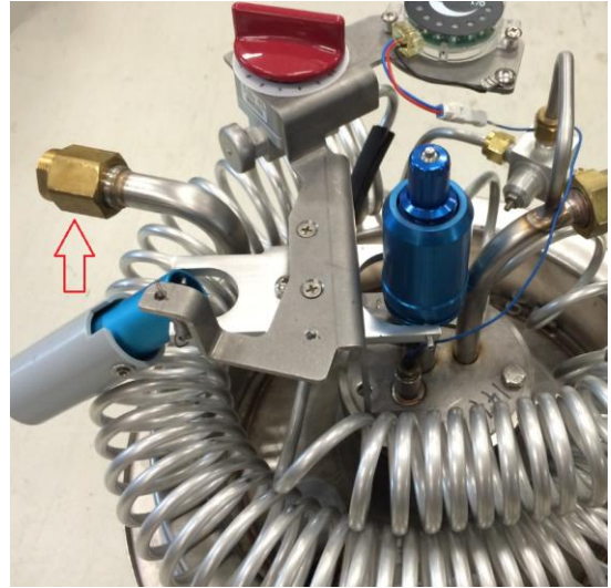
Figure 4. Newer Style Top Fill without Shroud
