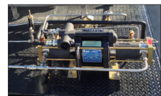
Booster Pump
