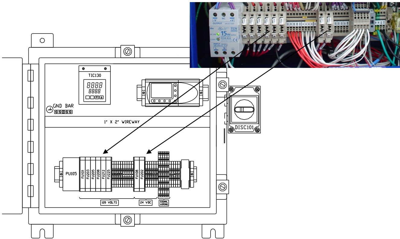
Figure 8 - Fuse Detail
