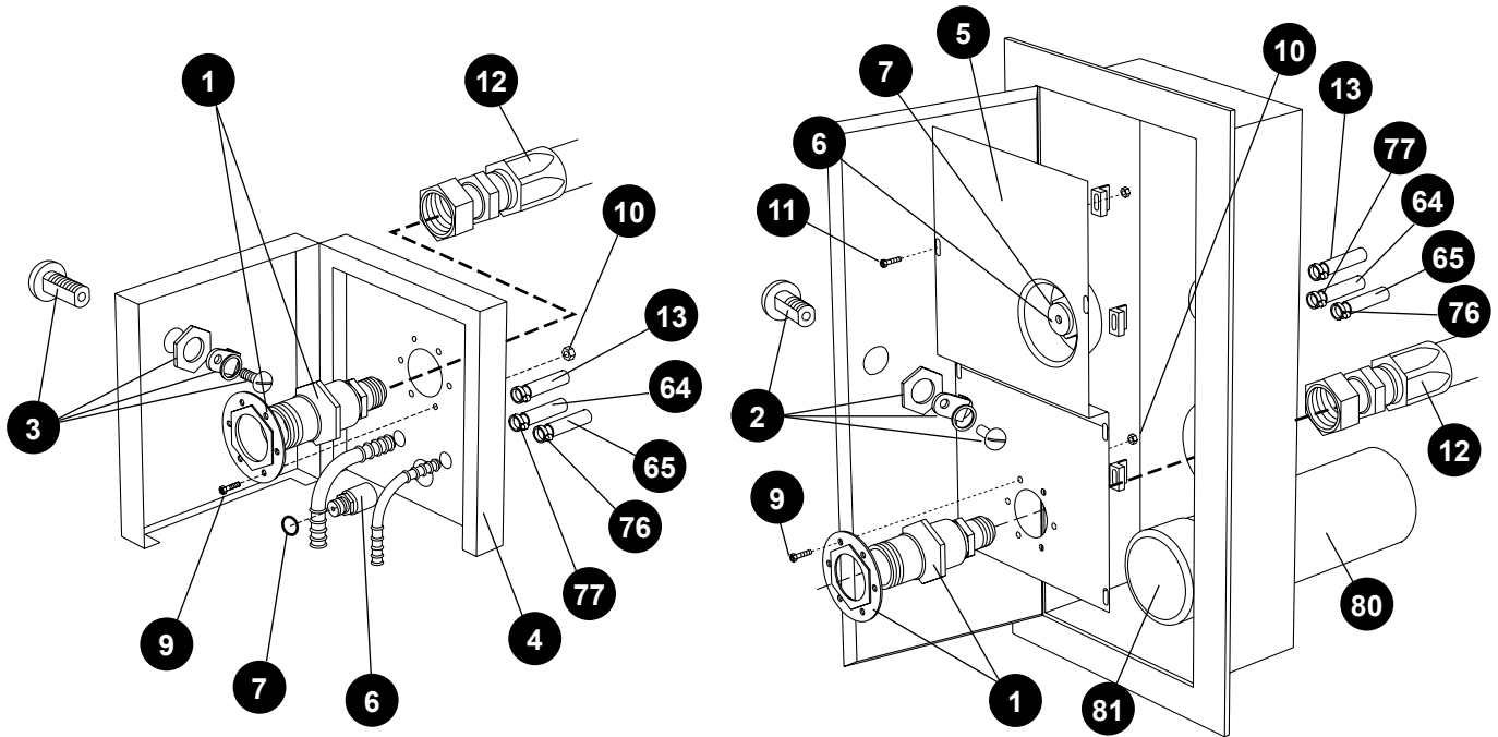
Flush Mount Fill Panel (With Fittings) (P/N 9722859)
