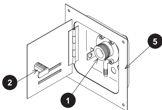
Flush-Mount Fill Box Part No. 9723139
